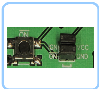
Module operating through ON and IGN pin outputs
