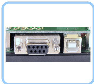
RS232 and USB communication ports
